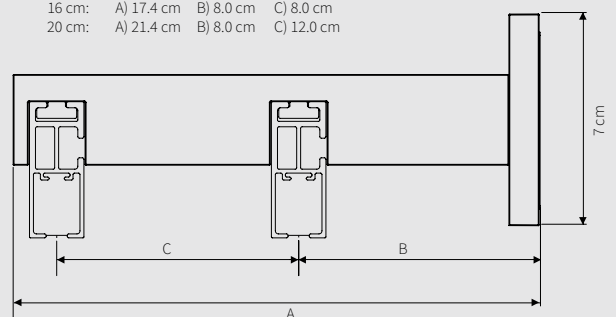
16 cm / 20 cm double wall bracket rectangular
