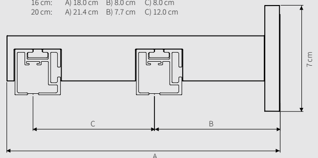
16 cm / 20 cm double wall bracket square
